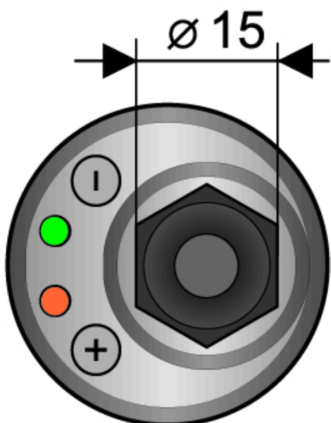
Dimensions (mm)
