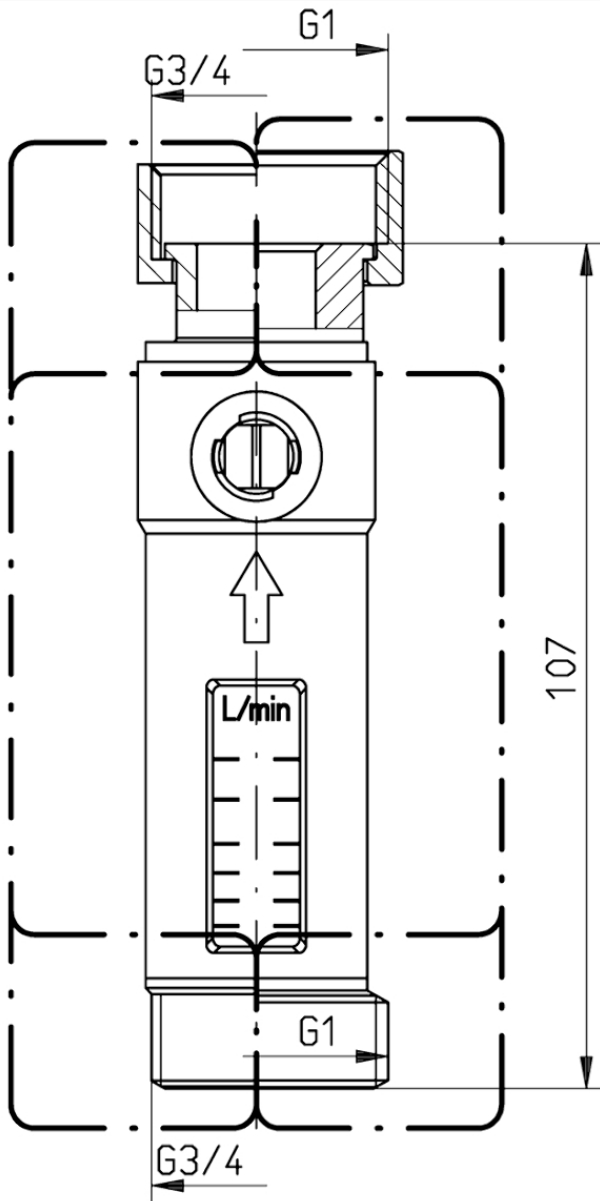
Dimensions (mm)
