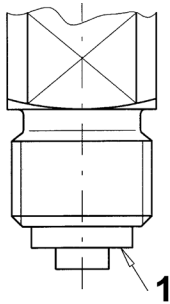
Fig. 4: Cylindrical threads
