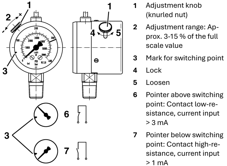
Fig. 9: Switching point
