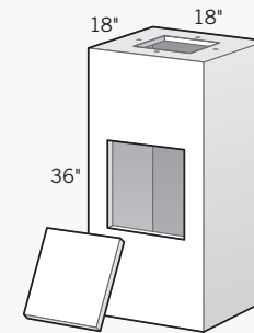
Column with End Cap 18"D × 18"L × 36"H Instantly build perfect stone or brick columns. Ships with access panel. Designed with top and bottom flange for attaching masonry anchor or bolting.
