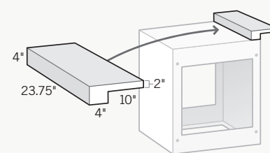
Straight Raised Backsplash Creates 4" high raised backsplash (23.75" long) with 10" cantilever and 14" counter surface. Requires 3 bolts for mounting (not included).
