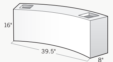
Curved Seating Wall (1/8 Circle) 8"D × 39.5"L × 16"H Curved seating wall has a 51" radius from the center point to the inside edge, perfect for pairing with our round fire pit.
