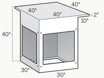
Bar-Height 90° Corner Cabinet with 10" Cantilever on Two Sides 30"D × 30"L × 40"H
