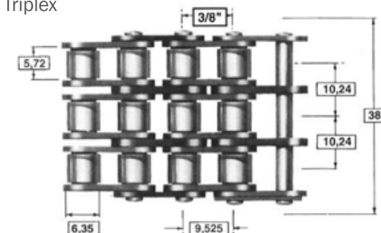
Triplex
