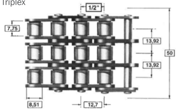
Triplex
