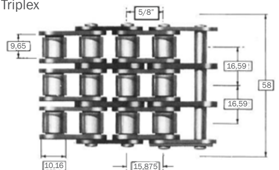
Triplex
