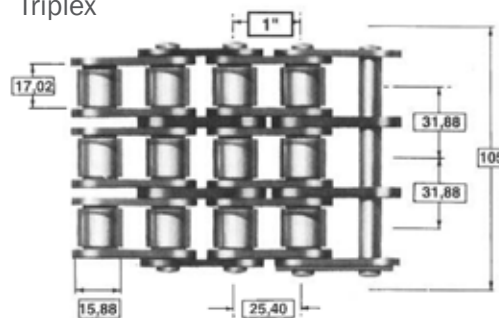
Triplex
