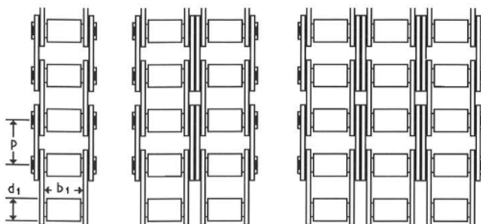
Simplex
