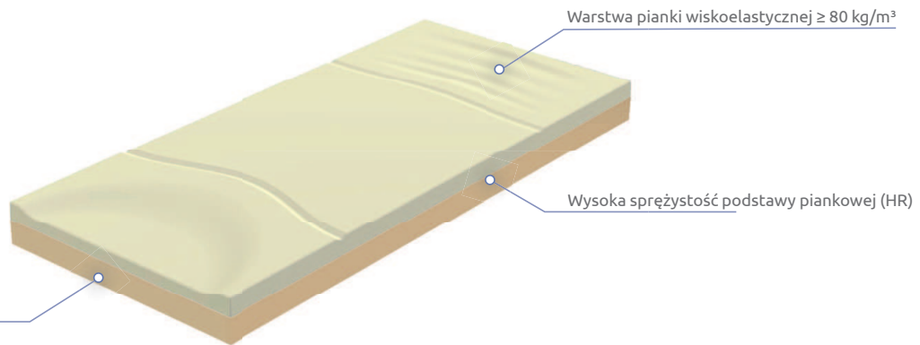
VMA62 model
