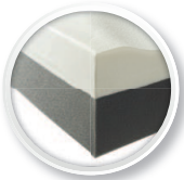
VMA62 model
