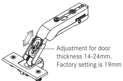
14mm door thickness with base plate height 0
