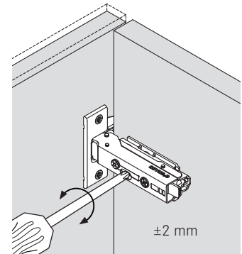
Height adjustment via base plate ±2.0mm via elongated hole ±2.5mm
