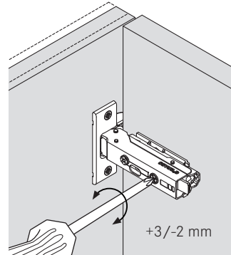
Depth adjustment via worm gear +3/-2 mm
