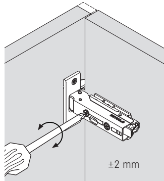
Side adjustment ±2 mm
