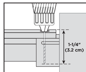
25. Using 9/64" bit provided, center into above holes and PREDRILL into top rail bracket at a depth of approximately 1-1/4". Use care to not drill through underside of top bracket.
