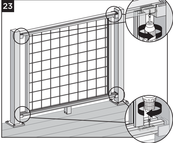
23. Attach L-Brackets to both top and bottom rails using one #8 x 5/8 flat head screw (provided).
