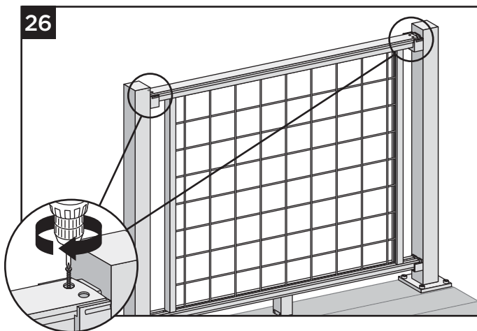
26. Install two #8 x 1-1/4" screws provided into top rail and top bracket on each end of top rail.
