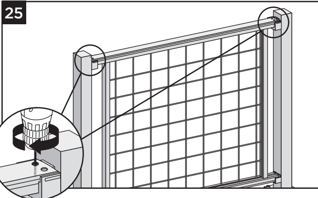
25. Using 9/64" bit provided, center into above holes and PREDRILL into top rail bracket at a depth of approximately 1-1/4". Use care to not drill through underside of top bracket.
