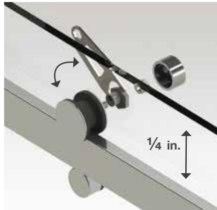
1/4 in. vertical adjustment for watertight closure
