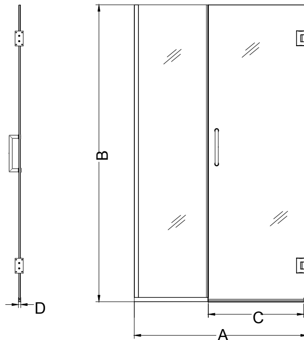
FRONT ELEVATION
