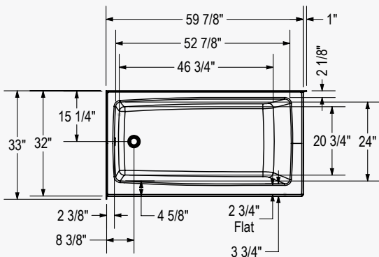
Mackenzie Corner 6032 - (Left drain version shown)
