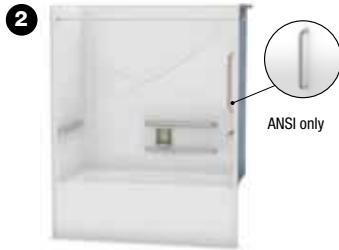
TUB SHOWER BASE MODEL WITH ADA OR ANSI GRAB BARS
