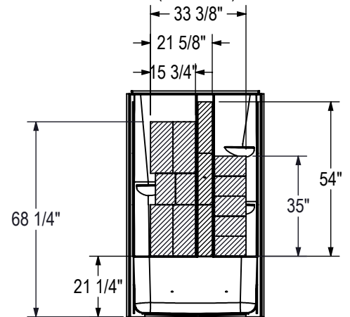
OPTIONAL REINFORCEMENT (Back Wall)
