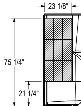
OPTIONAL REINFORCEMENT (Left shown)
