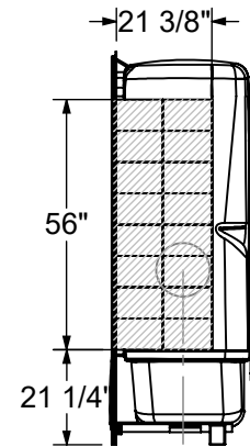
OPTIONAL REINFORCEMENT (Back Wall)
