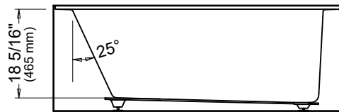
Back view
