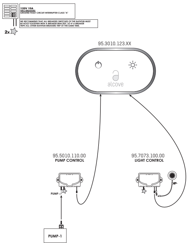
Fig. 22 Whirlpool and Chromotherapy light
