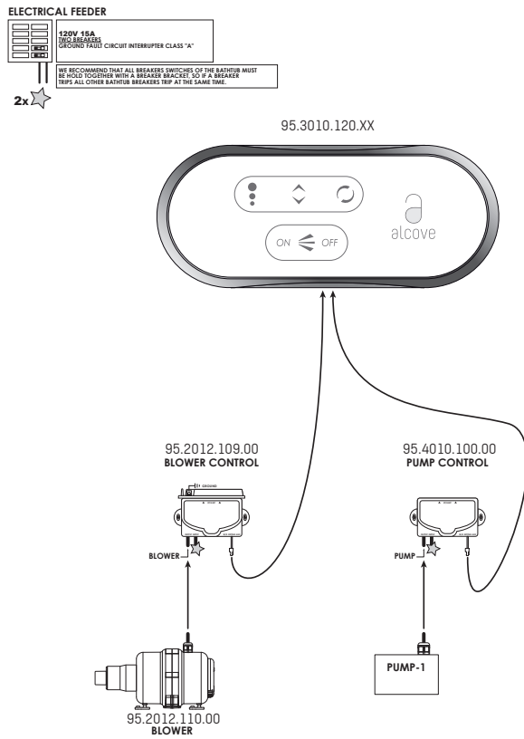
Fig. 25 Combined Whirlpool and Balne-Air or Vibro-Air
