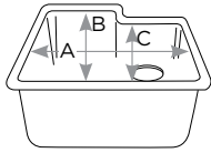
8" deep bowl A 22", B 18-1/4", C 15-5/16"
