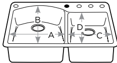
9" deep bowls A 15-1/4", B 18-3/8" C 12-7/8", D 16"
