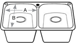
10" deep bowls A 14-1/8", B 18-7/8"
