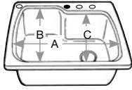
9" deep bowl A 21-1/8", B 17-5/8", C 15-5/8"
