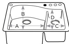
10" deep bowl, 7-1/2" deep bowl A 17-1/4", B 18" C 11", D 15-1/4"
