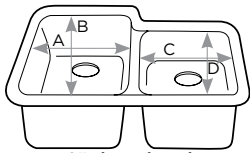
8" deep bowl A 14-1/2", B 18-1/8" C 14-1/2", D 15-5/8"
