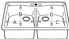
9" deep bowls A 14-1/2", B 17-1/8" C 14-1/2", D 17-1/8"
