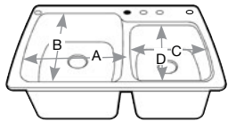
9" deep bowls A 14-1/4", B 18-7/8" C 13-3/4", D 15-1/4"
