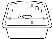
8-1/4" deep bowl A 18-7/8", B 18-1/8"
