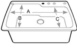
10" deep bowl A 29-1/2", B 18-3/4", C 16-1/4"
