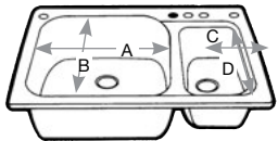
9" deep large bowl, 7" deep small bowl A 19-3/8", B 18-7/8" C 8-7/8", D 15-5/8"
