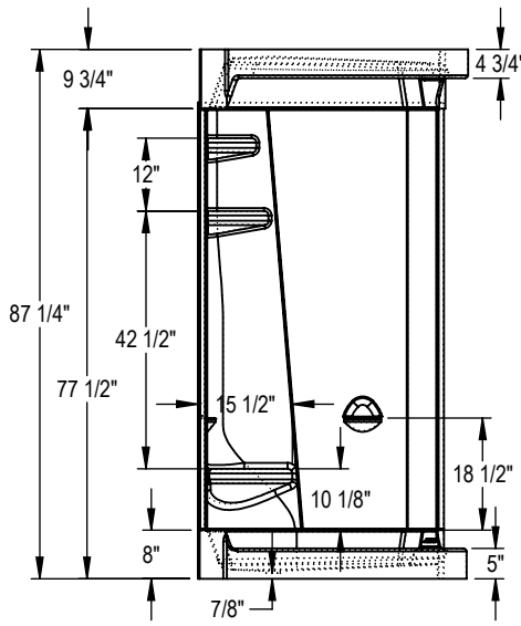
One piece with Seat
