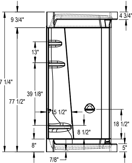
One piece with Footrest
