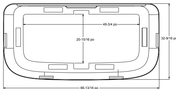
Coque
