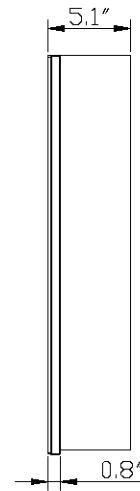
SIDE VIEW
