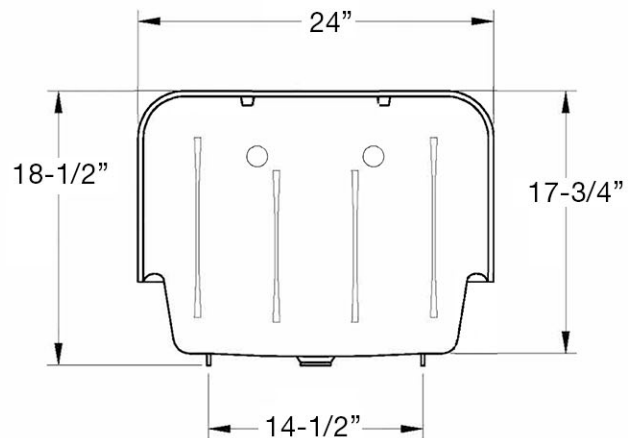
BACK VIEW
