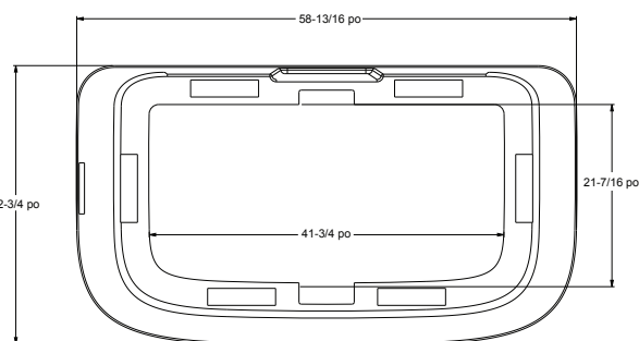
Coque
