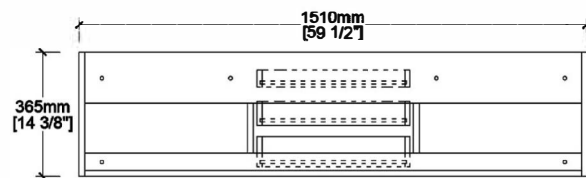
BACK VIEW
