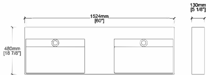
COUNTER-TOP VIEW
