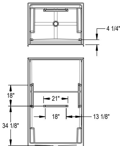
OPT. 18" Modern straight grab bar
