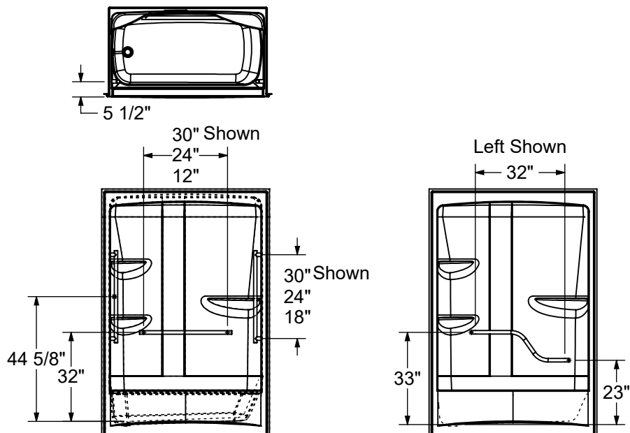
GRAB BAR (Left shown)
