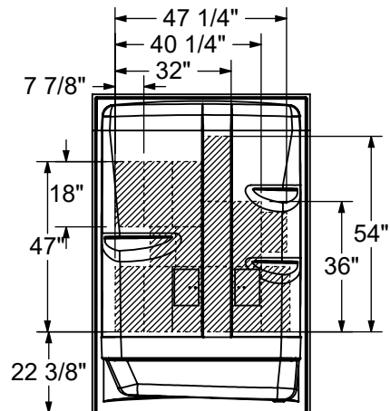
OPTIONAL REINFORCEMENT (Back Wall)
