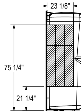
OPTIONAL REINFORCEMENT (Left shown)
