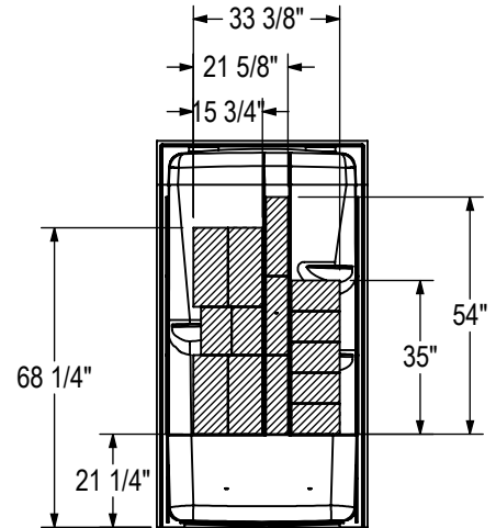
OPTIONAL REINFORCEMENT (Back Wall)
