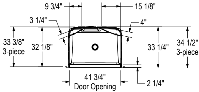
STANDARD 1-PIECE MODEL SHOWN
