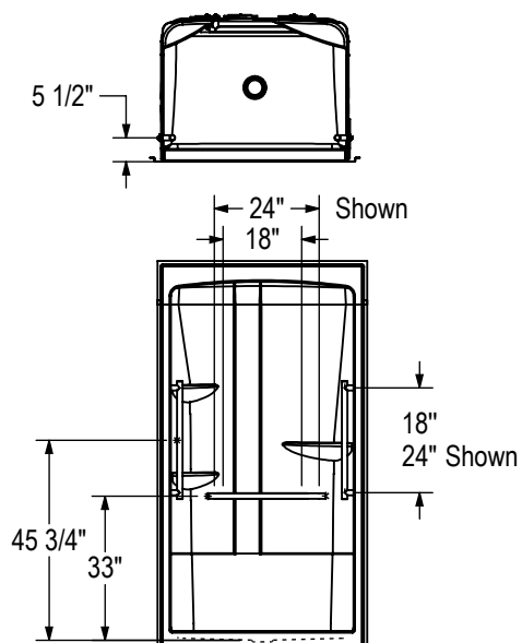
GRAB BAR (Left shown)
