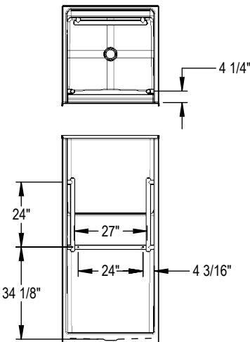
OPT. 24" Modern straight grab bar
