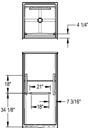
OPT. 18" Modern straight grab bar
