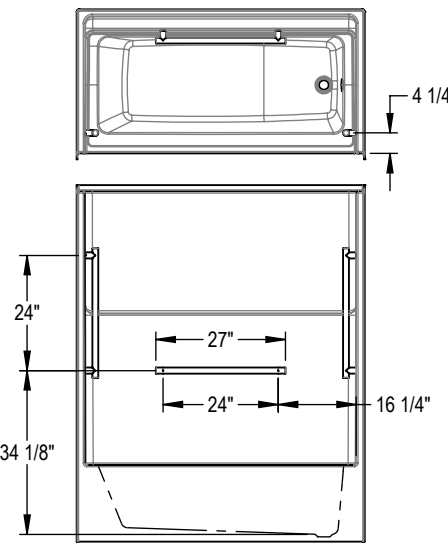
OPT. 24" Modern straight grab bar
