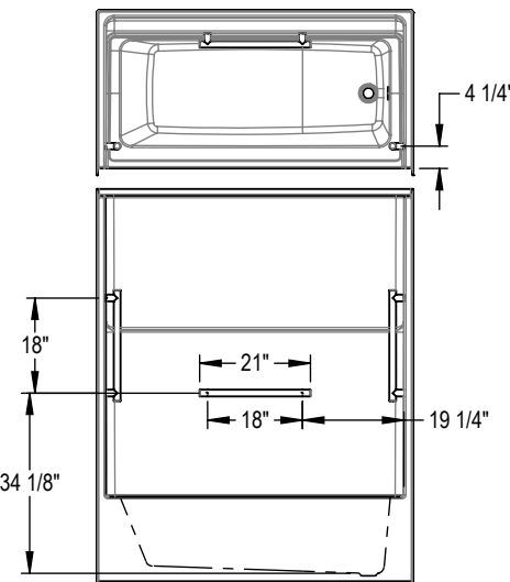
OPT. 18" Modern straight grab bar
