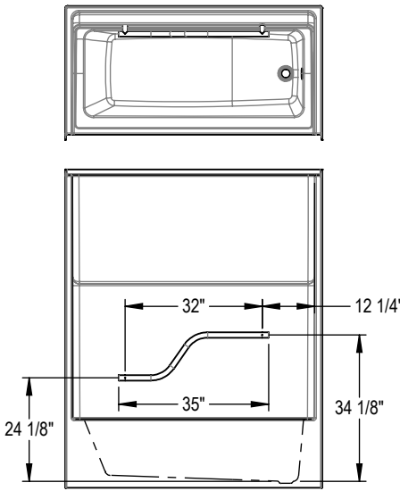
OPT. 32" curved grab bar (right shown)
