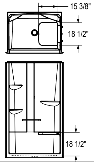
SEAT OPTION 20221 (1-Piece only)
