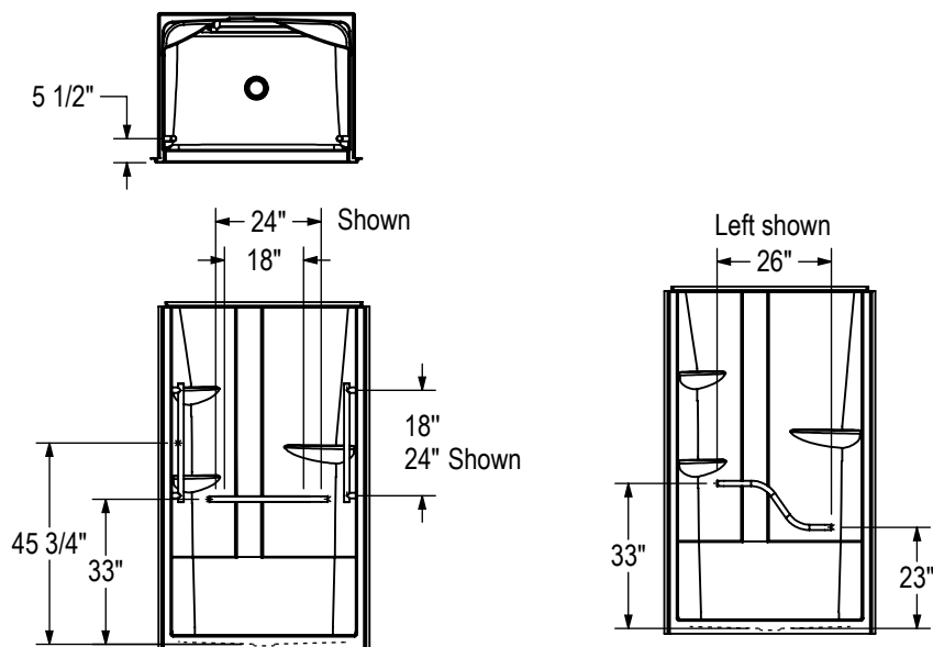
GRAB BAR (Left shown)
