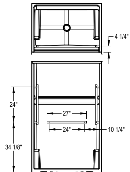
OPT. 24" Modern straight grab bar
