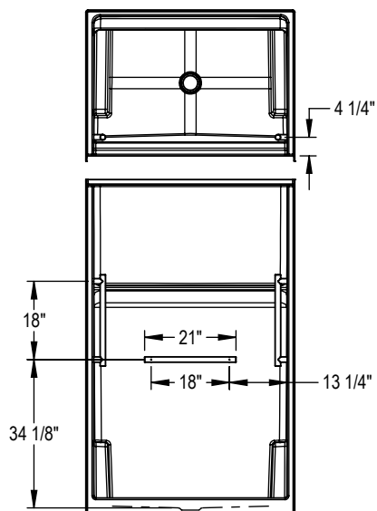
OPT. 18" Modern straight grab bar
