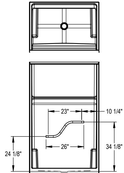
OPT. 23" curved grab bar (right-hand shown)
