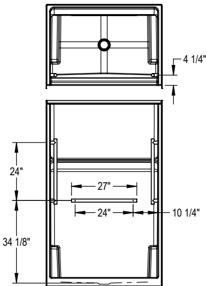
OPT. 24" Modern straight grab bar
