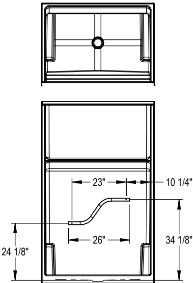
OPT. 23" curved grab bar (right-hand shown)
