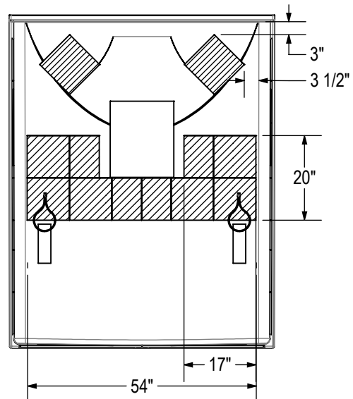
BACK WALL
