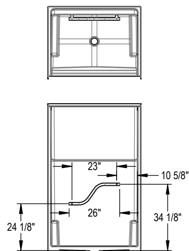
OPT. 23" curved grab bar (right-hand shown)
