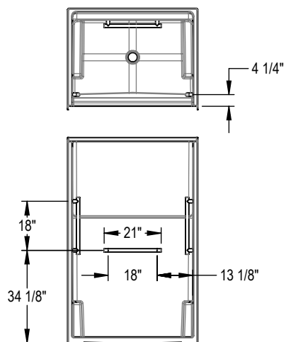
OPT. 18" Modern straight grab bar
