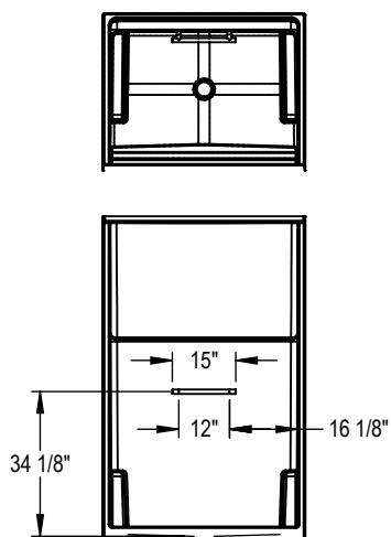
OPT. 12" Modern horizontal straight grab bar
