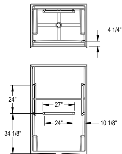
OPT. 24" Modern straight grab bar
