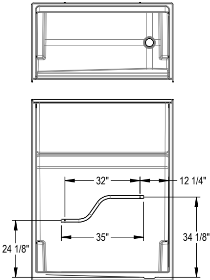
OPT. 32" curved grab bar (right-hand shown)
