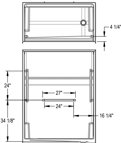
OPT. 24" Modern straight grab bar
