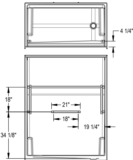
OPT. 18" Modern straight grab bar
