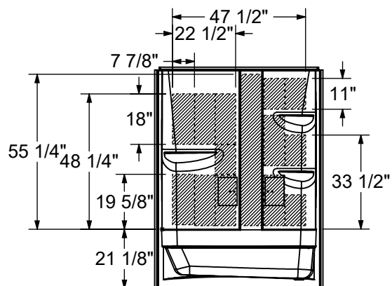
OPTIONAL REINFORCEMENT (Back Wall)
