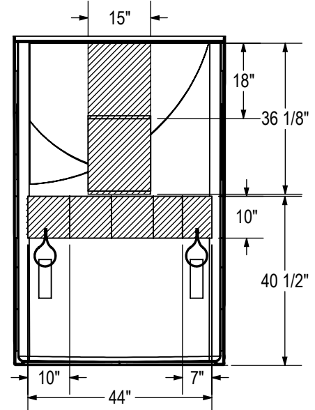
BACK WALL
