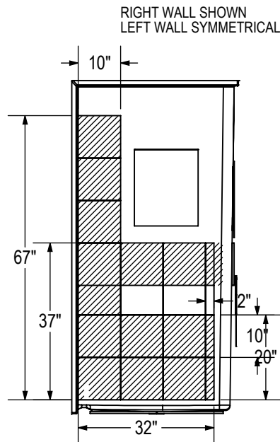
REINFORCEMENT BACKING
