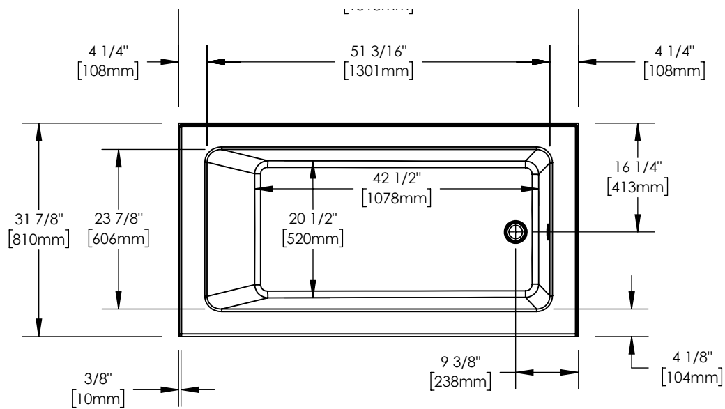
59 3/4" x 31 7/8" x 18 1/2" Bathtub
