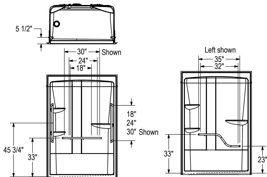
GRAB BAR (Left shown)
