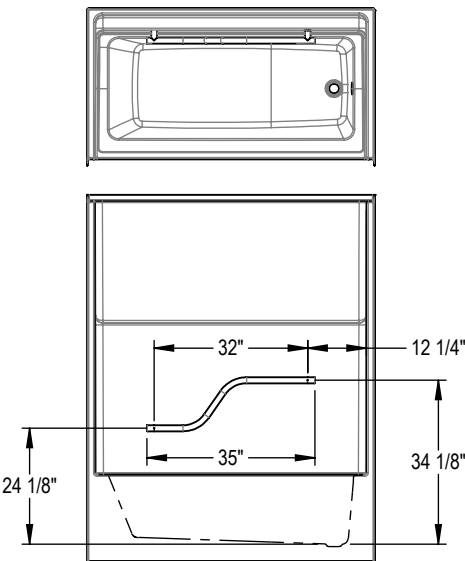
OPT. 32" curved grab bar (right shown)
