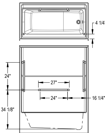
OPT. 24" Modern straight grab bar
