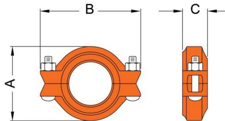
Model 7706 Reducing Coupling
