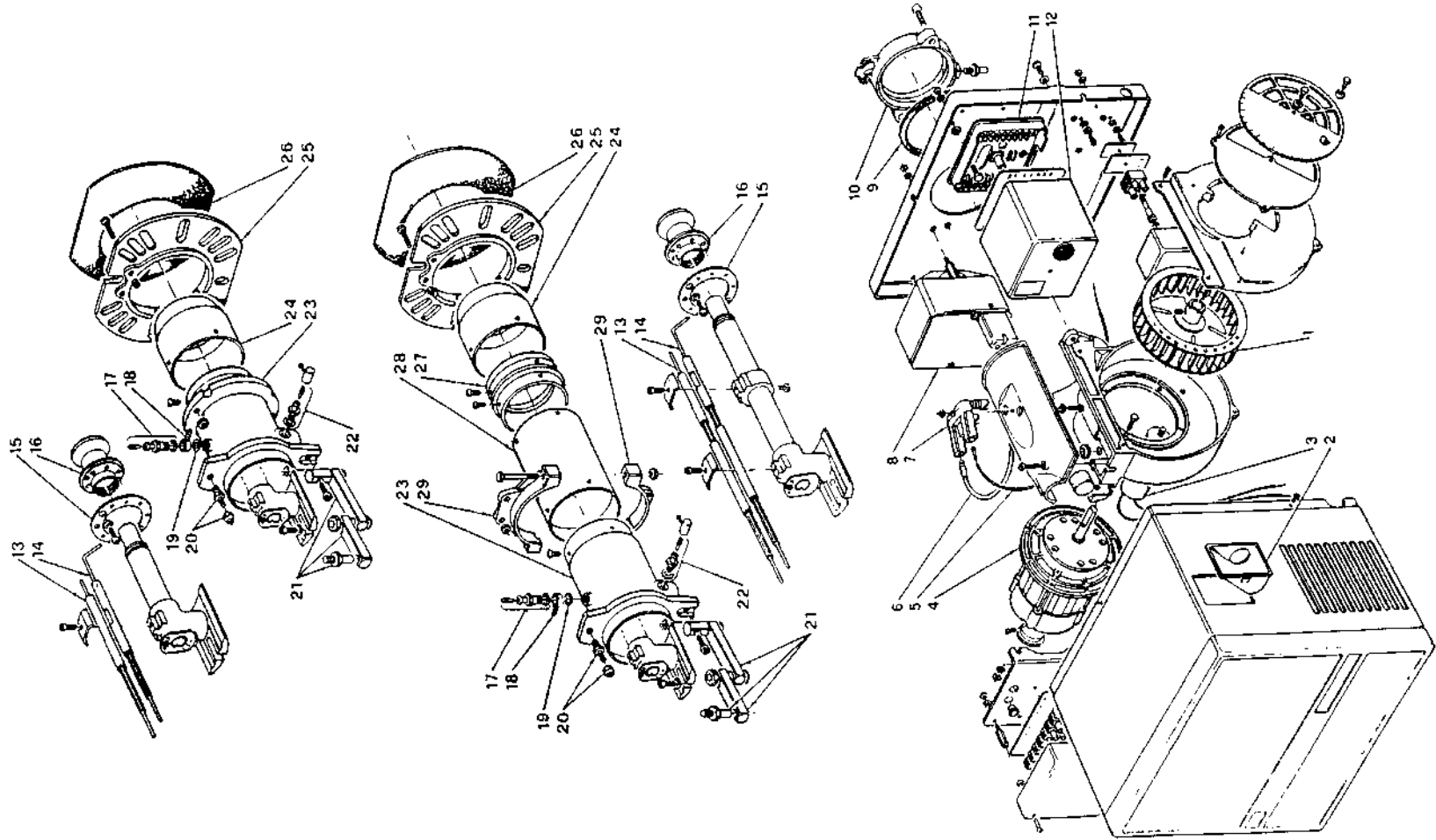
Riello Gas-2 Burner
