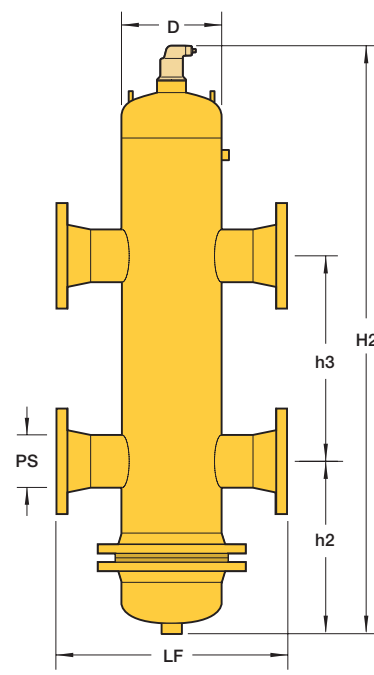
VXN Steel 2"-12" Flanged ASME with Removable Head
