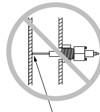
If probe is installed too close to boiler wall, an electrical short could occur.
