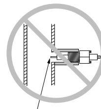
If probe is installed with extensions, an air pocket could develop shutting down the boiler. Debris could develop which can cause an electric short, rendering the low water cut-off ineffective.
