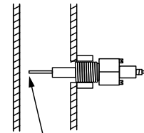
Make sure tip of probe is in pipe with 1/4" clearance from wall of pipe.
