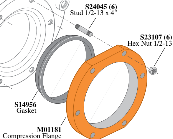
B56339 Suction Flange Kit For 8" O.D. Pipe
