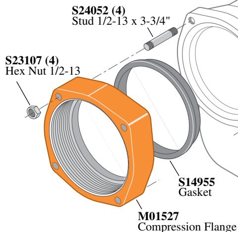
B50711 Discharge Flange Kit For 6" Standard Pipe
