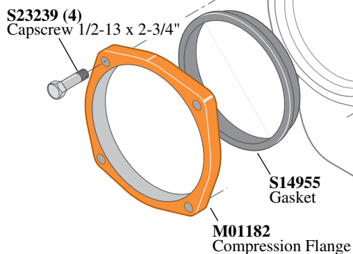
B56340 Discharge Flange Kit For 6" O.D. Pipe
