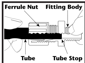
Ferrule Nut
