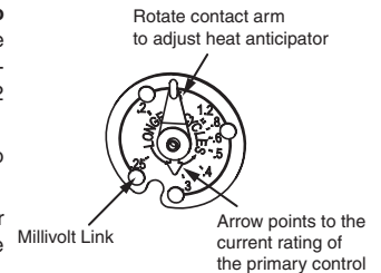
Figure 2. Anticipator adjustment
