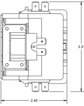
30 AMP MODEL (NO COVER)
