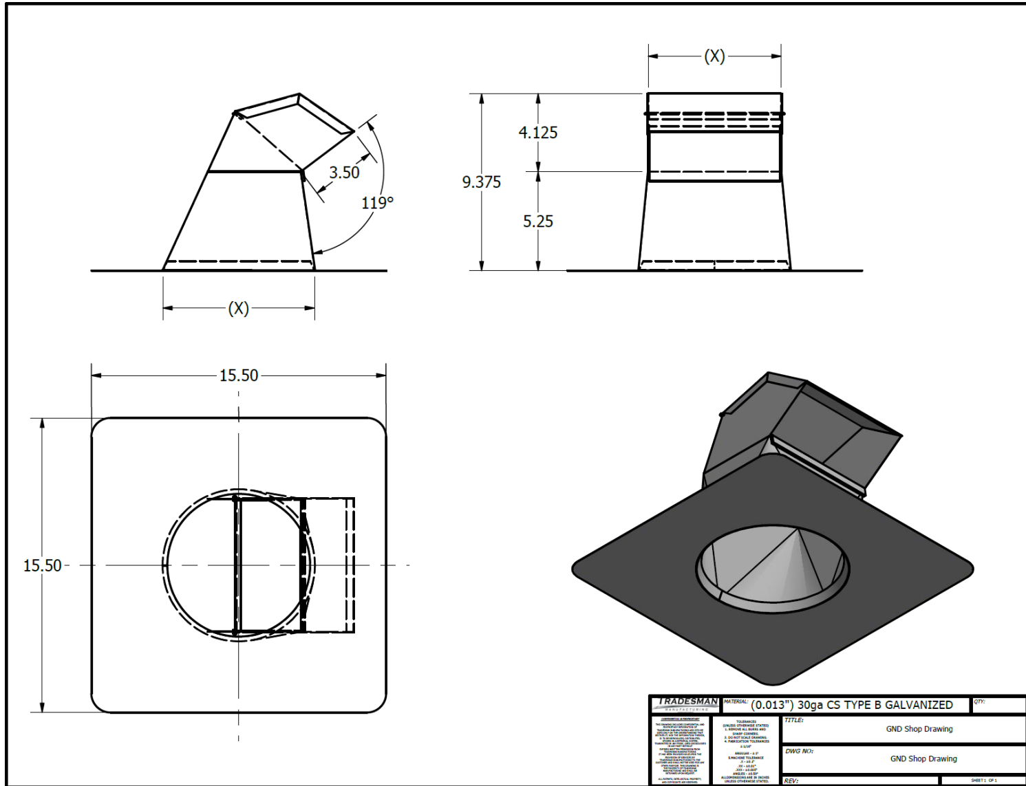
Gooseneck with Damper
