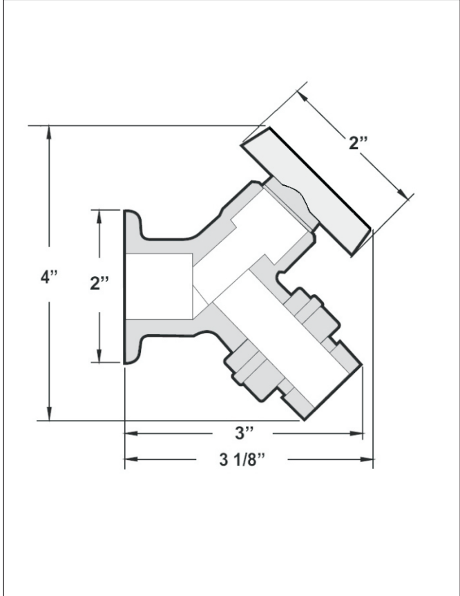
MHY-90 Series wall faucet dimensions
